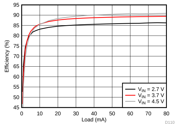
Figure 194. VPOS Efficiency
