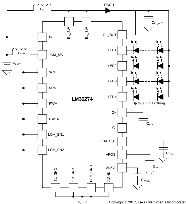
Simplified Schematic
